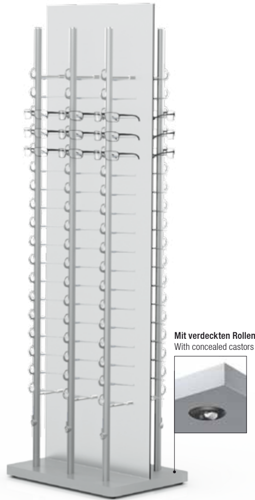
05 PG 6 620 x 1980 x 445 mm 108 / 144
