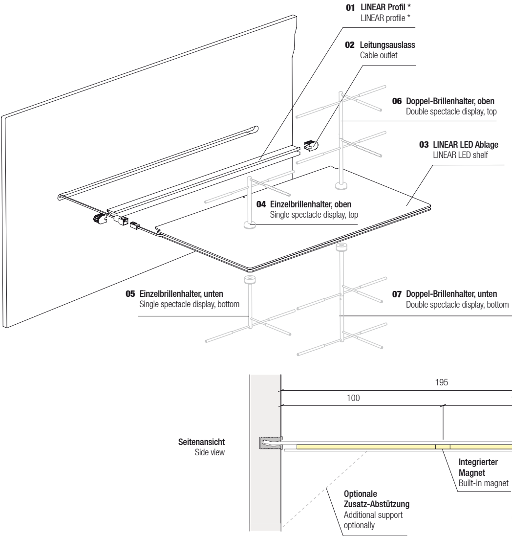
LED Ablagen nur 8 mm hoch! LED shelves only 8 mm thick!
