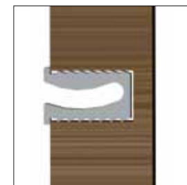
01. A LINEAR-Schiene in Holzpaneel LINEAR rail in wooden panel
